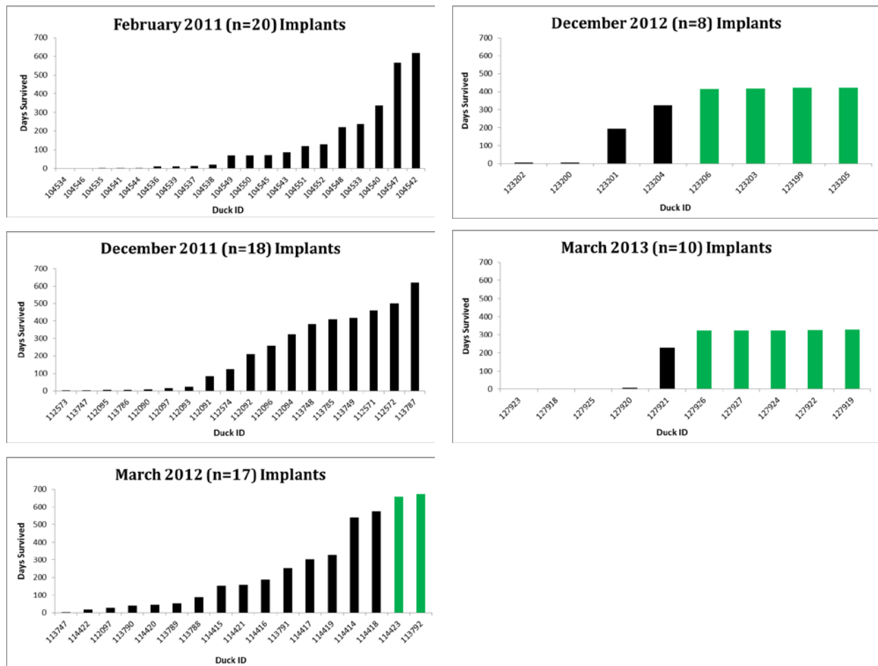
Figure 17. Number of days between release and 1 February 2014 that long-tailed ducks captured at Lake Ontario survived / transmitted data after being implanted with satellite transmitters. Green = online, black = dead or offline.
