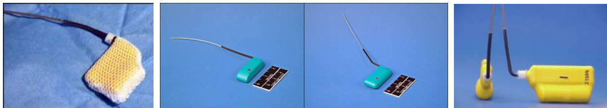
Figure 2. Implantable PTTs for use in sea ducks.
