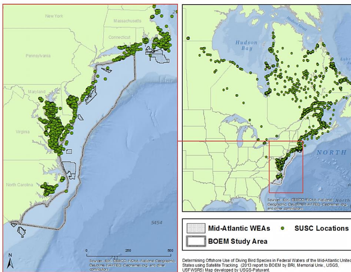
Figure 11. Best quality locations per duty cycle for 104 surf scoters (57 males, 47 females) marked during winter in Chesapeake Bay, MD/VA, Pamlico Sound, NC, and Narragansett Bay, RI relative to the proposed mid-Atlantic wind energy areas.
